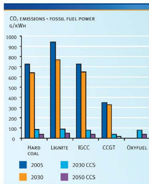
Figure 2 Emissions of fossil fuel power production
